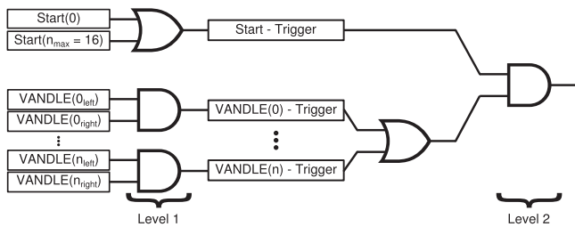
Fig. 12. A schematic of the on-board coincidence triggering used for the VANDLE system. Level 1 indicates the pairwise coincidences between PMTs on a VANDLE module. Level 2 represents the logical AND condition between VANDLE and the start detectors. The system can handle up to 16 start detectors and n VANDLE modules.
