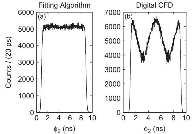
Fig. 4. The projection of the phase–phase diagrams for the FA and the DCFD, each case is for \Delta = 2 ns. The FA does not show any bias in the phase space, where as the DCFD is heavily biased because the response of the function is nonlinear in the interpolation region. The WAA produces a projection similar to that of the FA.
